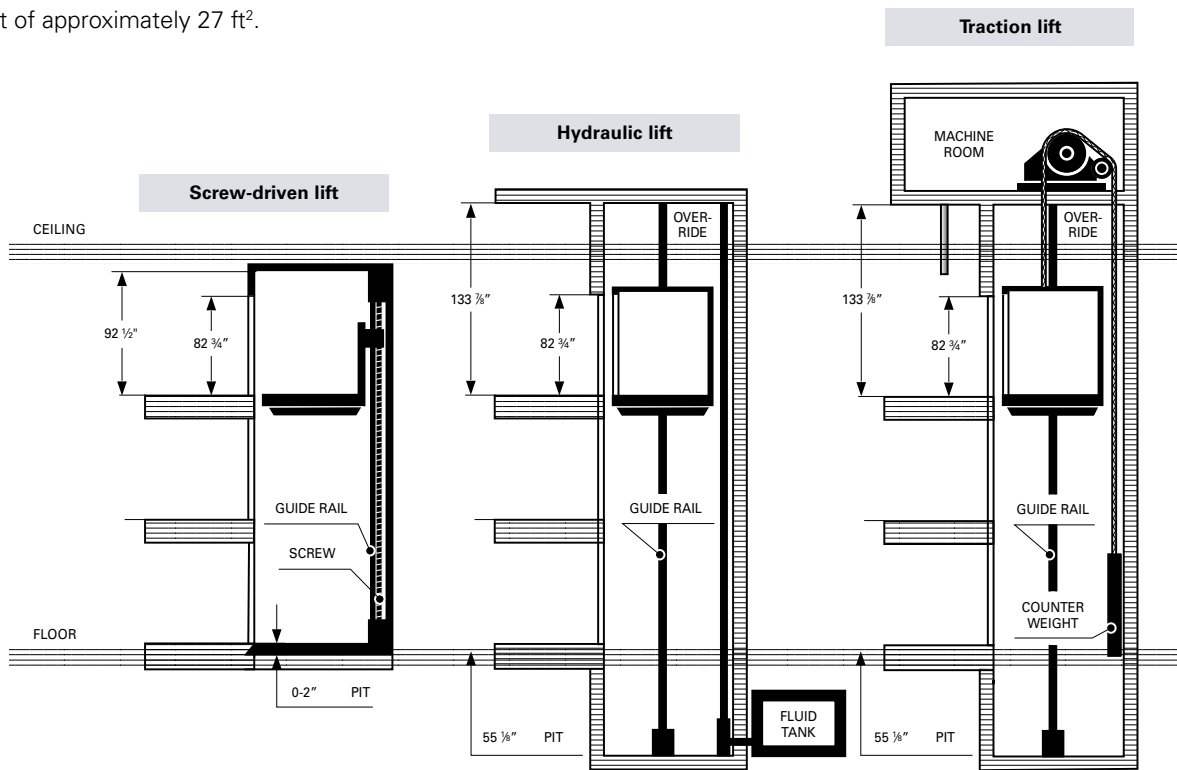
Unlike conventional lifts, Cibes screw-driven lifts do not require a lot of space above and beneath the lift.
